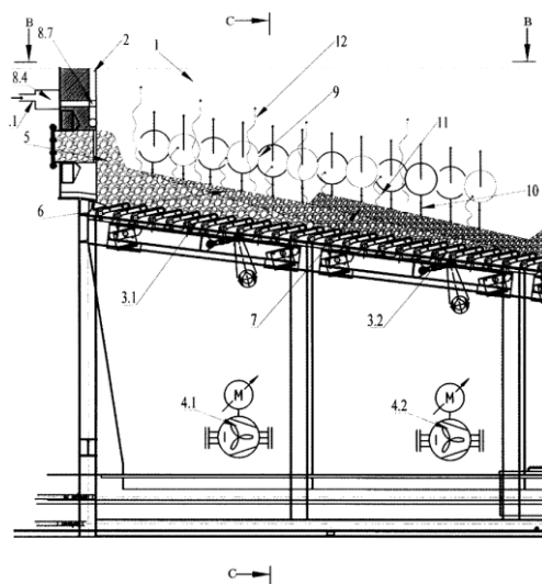
(54) THERMOBIOGAS BOILER GENERATOR CREATED BY RADIATION FROM THE FLAME ZONE
