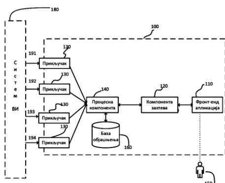
(54) SYSTEM AND PROCEDURE FOR REASONING DECISIONS IN ARTIFICIAL INTELLIGENCE-BASED SYSTEMS
