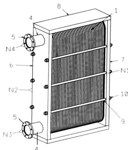
(54) PLATE HEAT EXCHANGER FOR HEAT RECOVERY FROM GASES
