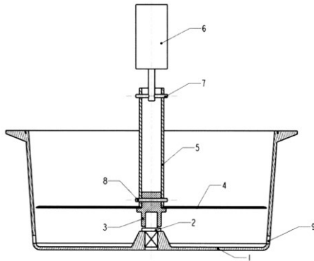
(54) METHOD AND DEVICE FOR PEELING ROOT VEGETABLES IN THE SINK
