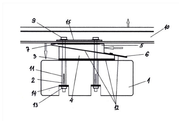
(54) WEDGE RAILWAY FASTENER
