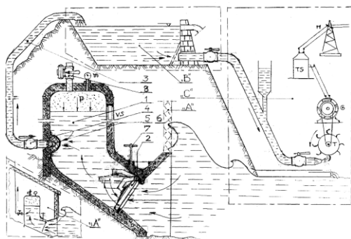
(54) A PLANT FOR RAISING SEAWATER TO A HIGHER LEVEL USING THE ENERGY OF SEA WAVES
