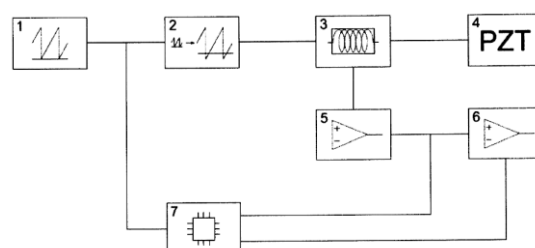
(54) PROCEDURE FOR PRECISE POSITIONING OF A PIEZO ELEMENT IN RELATION TO A REFERENCE SURFACE OR MEASURING THE DISTANCE BETWEEN A PIEZO ELEMENT AND A REFERENCE SURFACE WITHOUT THE USE OF SENSORS OR DISTANCE MEASURING DEVICES
