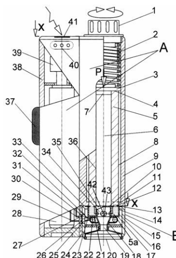
(54) WAX MELTING DEVICE
