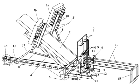
(54) AN EXERCISE MACHINE WITH THREE SUPPORTS
