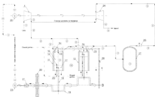
(54) GAS-TURBINE POWER-PLANT WITH PNEUMATIC MOTOR WITH ISOBARIC INTERNAL COMBUSTION
