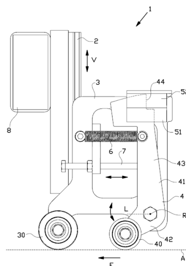
(54) HEIGHT DETECTION DEVICE FOR DETECTING A HEIGHT OF A TIRE COMPONENT
