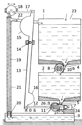
(54) HYDRO-MECHANICAL MOTOR
