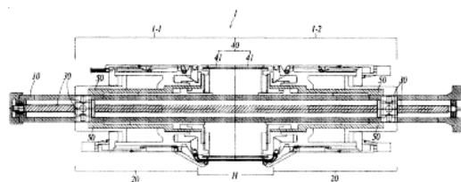
(54) TIRE BUILDING DRUM
