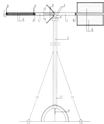
(54) BUTTERFLY VERTICAL AXIS WIND TURBINE
