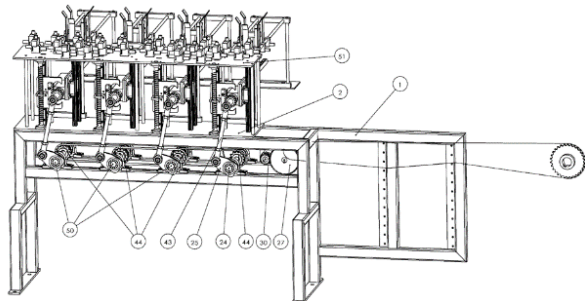
(54) DEVICE FOR AUTOMATIC ARRANGING WOODEN SLATS ON THE CONVEYOR BELT PRODUCTION LINE
