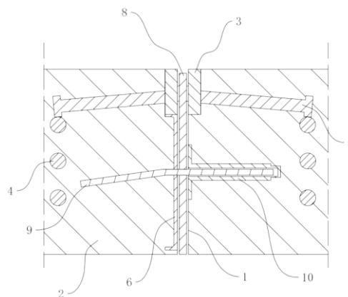
(54) EXPANSION JOINT STRUCTURE FOR CONCRETE FLOOR
