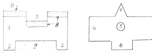
(54) SPECIAL BRICKS FOR UNDERGROUND ROAD HEATING
