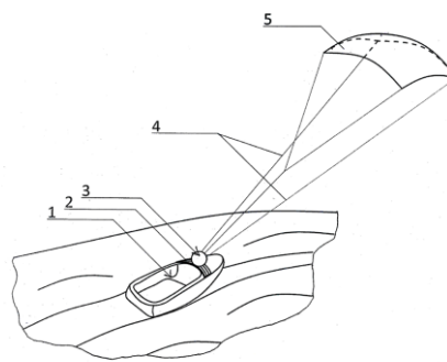
(54) CONTROL AND PROPULSION UNIT WITH A TRACTION KITE, AS WIND DRIVE, INTENDED FOR A VESSEL OR VEHICLE
