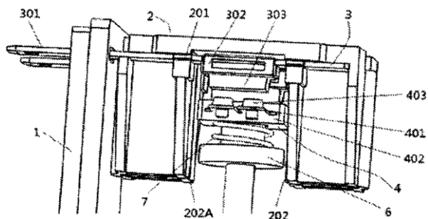
(54) RELAY HAVING HIGH RELIABILITY AND HIGH VIBRATION RESISTANCE
